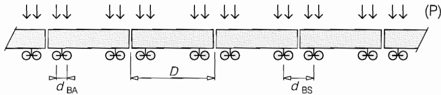
Figure E2 - Conventional train
